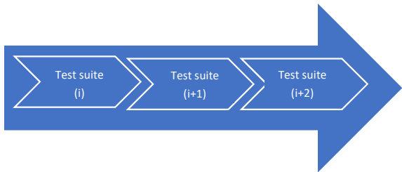
Legacy Architecture
