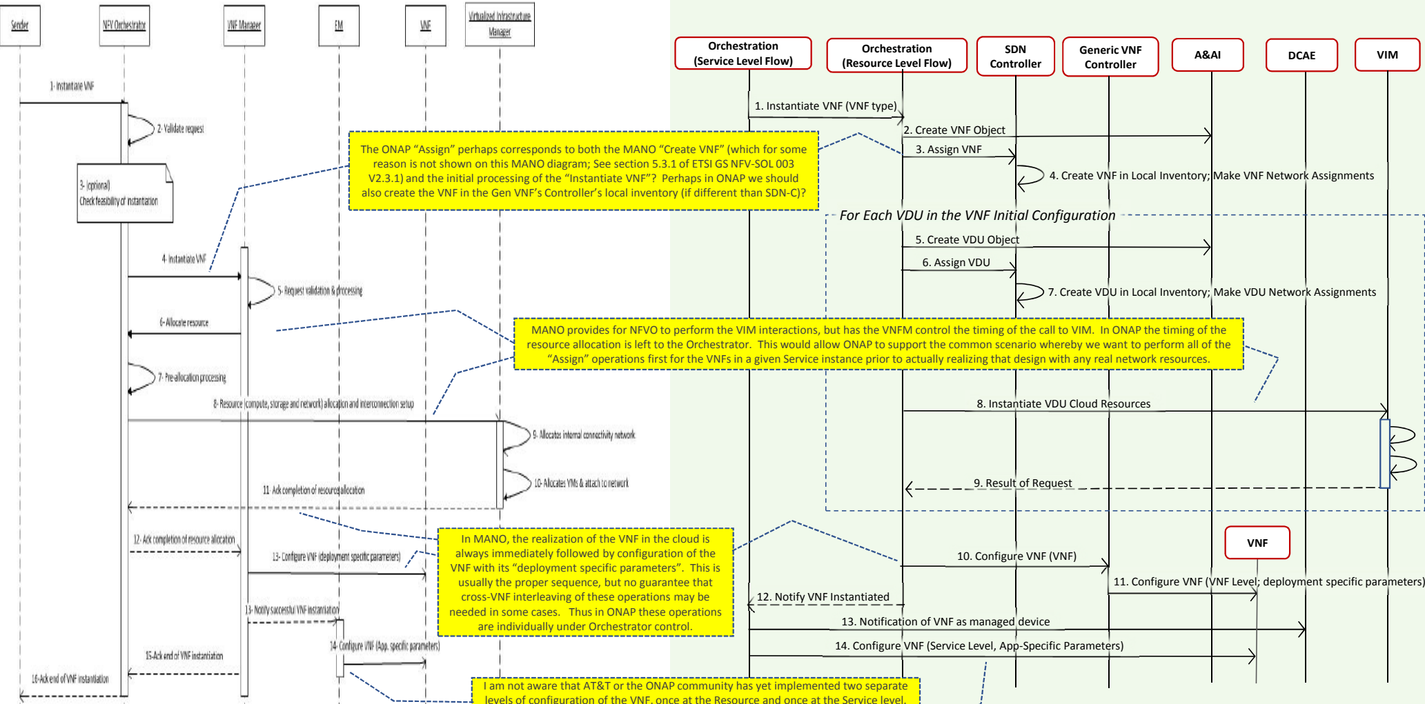
Figure B.9: VNF instantiation message flow
