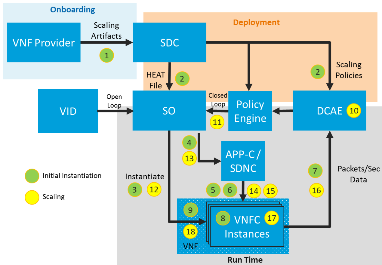
Figure 3: High level overview of scale-out workflow
